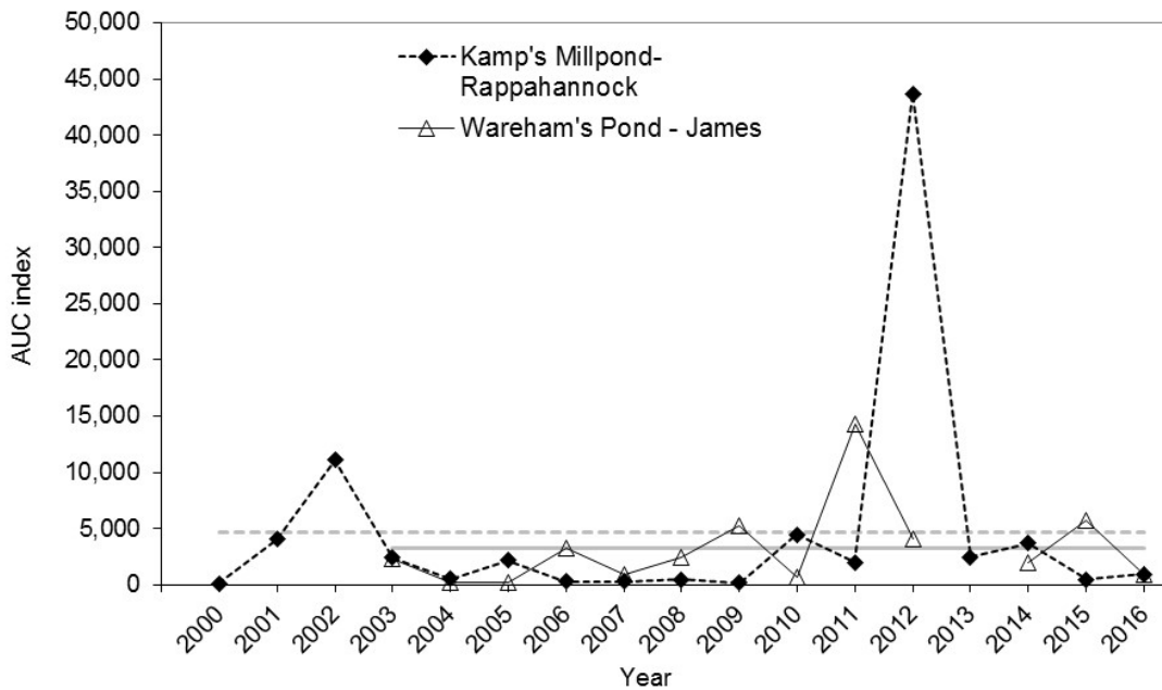
Figure 3. Abundance indices and time series average calculated by the area-under-the-curve method for glass eels from Wareham's Pond (James River system) and Kamp's Millpond (Rappahannock River system). Time series averages are shown as solid (Wareham's Pond) and dotted (Kamp's Millpond) lines.
