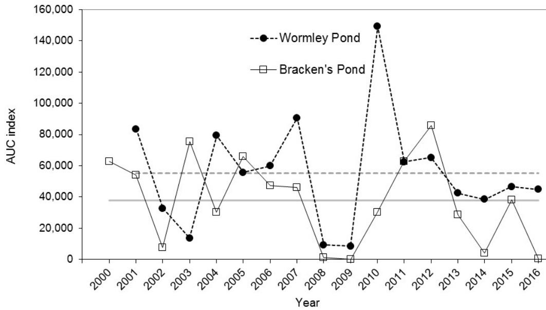
Figure 2. Abundance indices and time series average calculated by area-under-the-curve method for glass eels from Wormley Pond and Bracken's Pond (York River system). Time series averages are shown as solid (Bracken's Pond) and dotted (Wormley Pond) lines.
