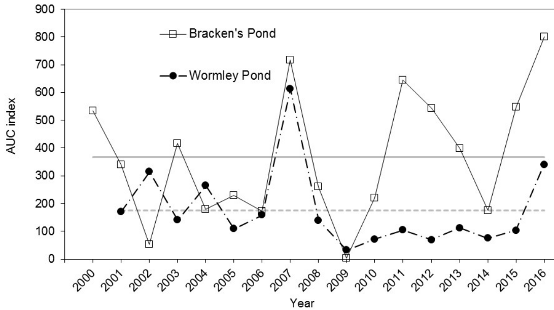
Figure 4. Abundance indices and time series average calculated by the area-under-the-curve method for elvers from Wormley Pond and Bracken's Pond (York River System). Time series averages are shown as solid (Bracken's Pond) and dotted (Wormley Pond) lines.
