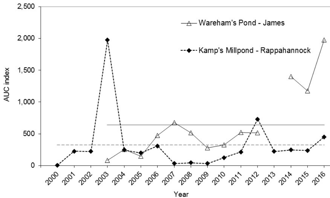
Figure 5. Abundance indices and time series average calculated by the area-under-the-curve method for elvers from Wareham's Pond (James River system) and Kamp's Millpond (Rappahannock River system). Time series averages are shown as solid (Wareham's Pond) and dotted (Kamp's Millpond) lines.
